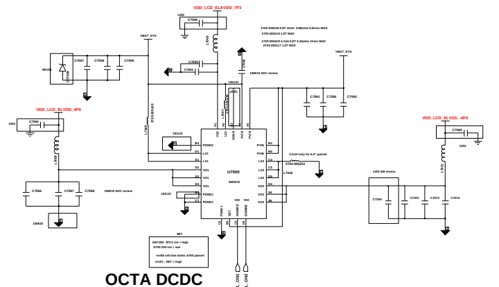
OCTA DCDC
