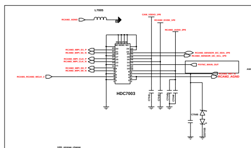
RCAM2_5M CAMERA(24PIN)_GC5035
