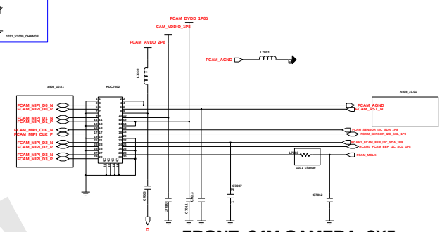
FRONT_24M CAMERA_2X5
