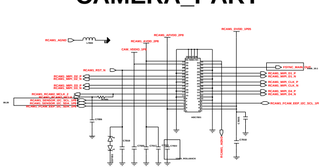
RCAM1_24M CAMERA(34PIN)_IMX576
