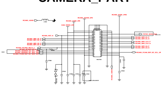
RCAM1_24M CAMERA(34PIN)_IMX576
