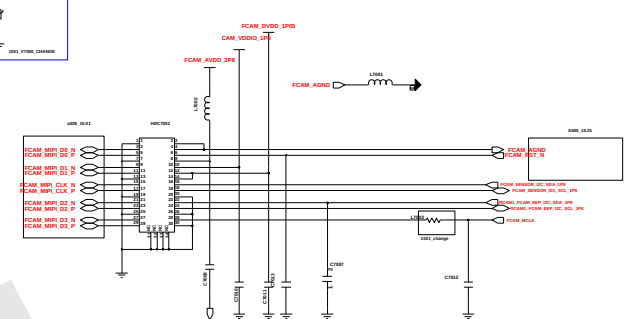
FRONT_24M CAMERA_2X5
