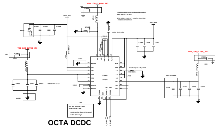
OCTA DCDC
