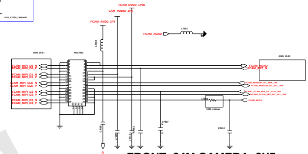
FRONT_24M CAMERA_2X5
